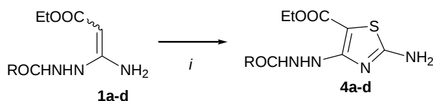
Scheme 4. Reagents and conditions: i , thiourea / Br 2 / AcOH, 0 - 5 °C.
