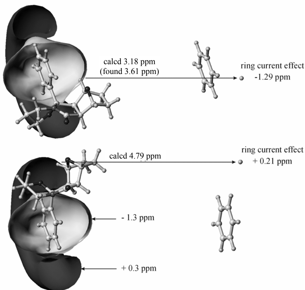
Figure 2 Ring current effect on H-3 in 7c
