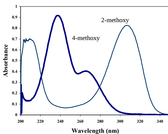
Figure 3. UV spectra of 2-methoxy- ( 6a , thin line) and 4-methoxy- ( 6b , thick line) 3,5-dimethylthiotetronic acid, recorded in MeOH at 25 °C.
