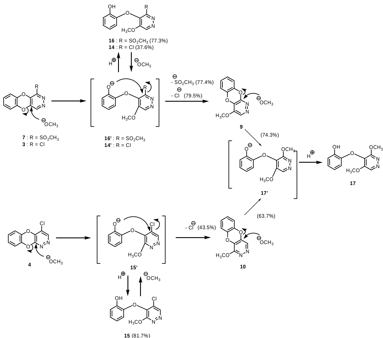
Scheme 3
