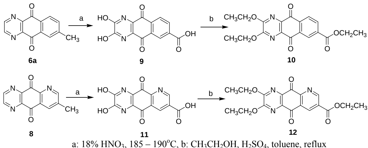
Scheme 2. Oxidation of benzo- or pyridoquinoxalinediones.
