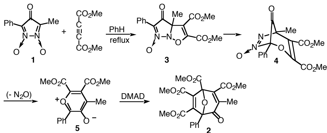
Scheme 1. Proposed origin of 2
