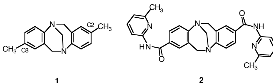
Figure 1. Tröger's base and an example of molecular receptors.
