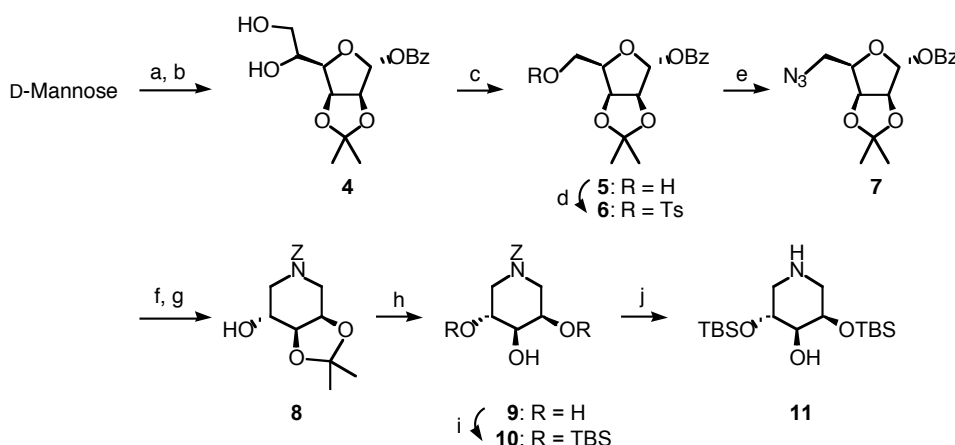
Scheme 1. Reagents and conditions: (a) (i) anhydrous CuSO 4 , acetone, conc. H 2 SO 4 , (ii) BzCl, pyridine (86% in 2 steps); (b) 70% aq. AcOH (quant); (c) (i) NaIO 4 , Et 2 O, H 2 O, (ii) NaBH 4 , MeOH (64% in 3 steps); (d) TsCl, pyridine (75%); (e) NaN 3 , DMF (72%); (f) 1 N aq. NaOH, MeOH (97%); (g) (i) H 2 , cat. Pd(OH) 2 , MeOH, (ii) CbzCl, Et 2 O, sat. aq. NaHCO 3 (87% in 2 steps); (h) 80% aq. AcOH, 90°C (92%); (i) TBSCl, Et 3 N, DMF (87%); (j) H 2 , cat. 10% Pd/C, MeOH (71%).
