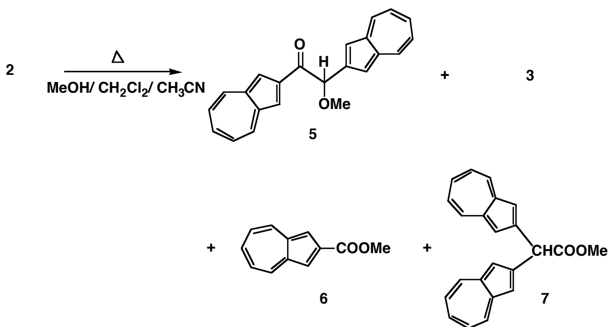
Scheme 2
