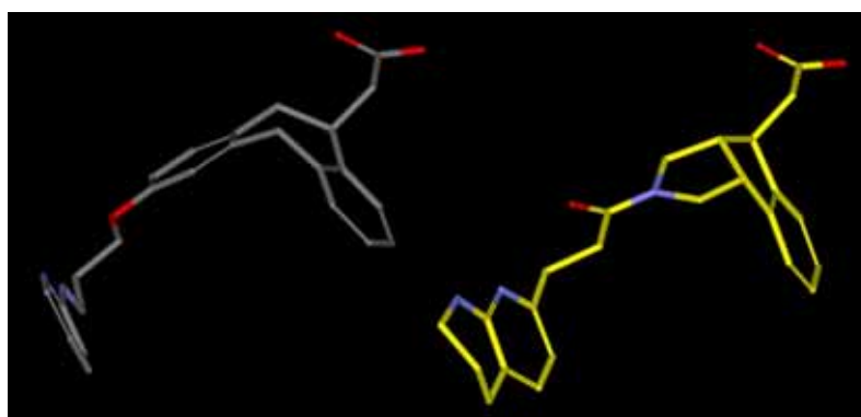
Figure 3. Comparison of the Right Turn Conformations of SB-265123 (gray) and 14ab (yellow).
