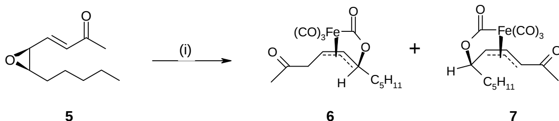
Scheme 2. (i) \text{Fe}_2(\text{CO})_9 , THF, rt, 3 h, 64%, 7 : 6 in a 4 : 1 ratio.
