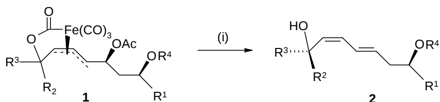
Scheme 1. (i) Li naphthalenide, THF, -78^{\circ}\text{C} \rightarrow \text{rt} , 17 h, 66-97%.
