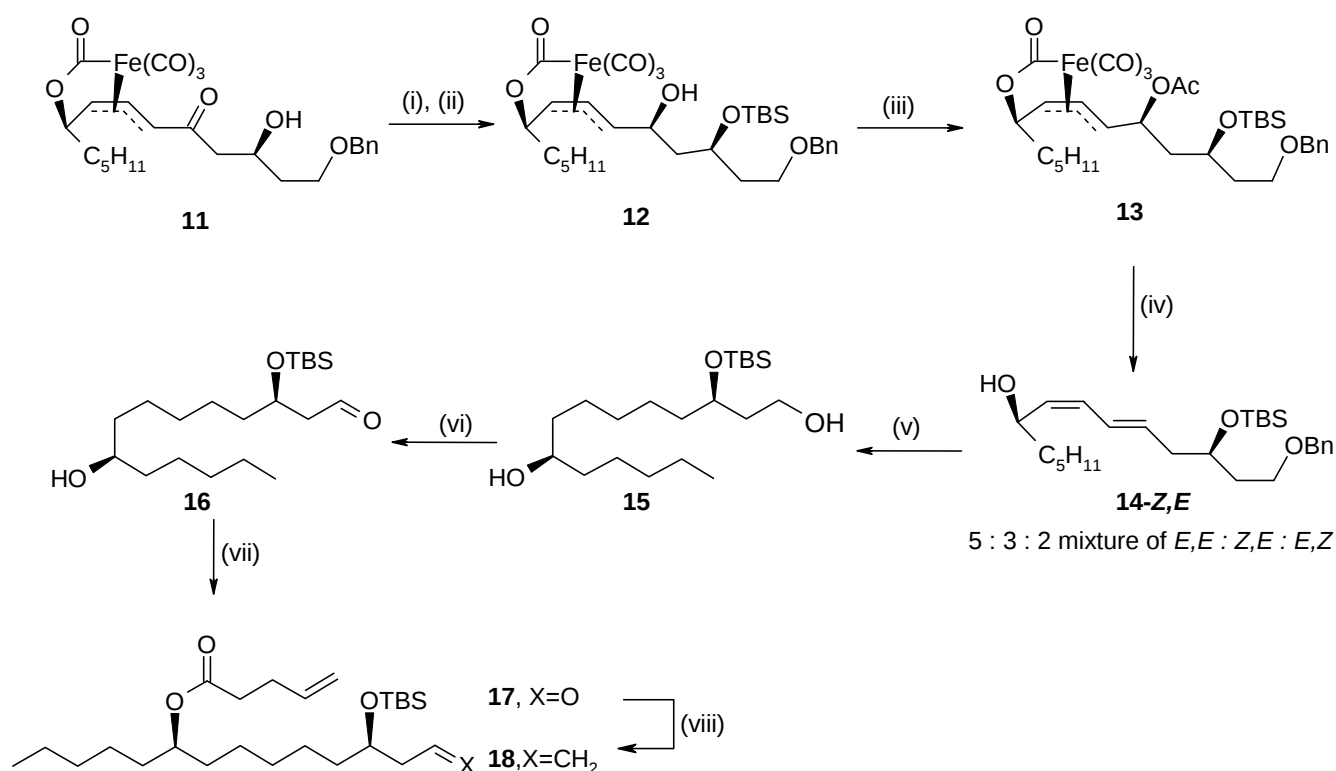
Scheme 4. Reagents and conditions: (i) TBSOTf, \text{Et}_3\text{N} , \text{CH}_2\text{Cl}_2 , 0^{\circ}\text{C} , 18 h, 100%; (ii) i - \text{Bu}_3\text{Al} (1M solution in toluene), \text{CH}_2\text{Cl}_2 , 0^{\circ}\text{C} , 30 min, 83%; (iii) \text{Ac}_2\text{O} , \text{Et}_3\text{N} , DMAP, \text{CH}_2\text{Cl}_2 , 0^{\circ}\text{C} \rightarrow \text{rt} , 2h, 98%. (iv) Li naphthalenide, THF, -78^{\circ}\text{C} \rightarrow \text{rt} , 17 h, 98%; (v) Pd/C, \text{H}_2 , EtOAc, 12 h, 83%; (vi) \text{RuCl}_2(\text{PPh}_3)_3 , benzene, \text{K}_2\text{CO}_3 (2 eq.), rt, 20 h, 78%; (vii) 4-pentenoyl chloride, DMAP (6 eq.), \text{CH}_2\text{Cl}_2 , 0^{\circ}\text{C} \rightarrow \text{rt} , 3 h, 65%; (viii) (\text{Ph})_3\text{PCH}_3\text{Cl} , t -BuOK, THF, 0^{\circ}\text{C} \rightarrow \text{rt} , 85%.
