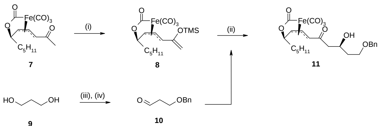
Scheme 3. (i) TMSOTf, \text{Et}_3\text{N} , \text{CH}_2\text{Cl}_2 , 0°C, 1 h, 84%; (ii) \text{OHC}(\text{CH}_2)_2\text{OBn} ( 10 ), \text{BF}_3 \cdot \text{OEt}_2 , \text{CH}_2\text{Cl}_2 , -78°C then \text{Et}_3\text{N} , HF-pyr, THF, 63%; (iii) \text{BnBr} , THF, TBAI, \text{NaH} , rt, 16 h, 73%; (iv) DMSO, (\text{COCl})_2 , \text{CH}_2\text{Cl}_2 , \text{NEt}_3 , -78°C \rightarrow rt, 1.5 h, 69%.
