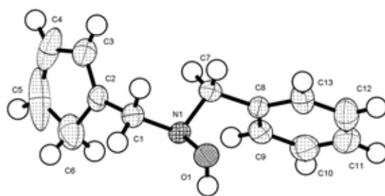
Figure 1. X-ray crystal structure for compound(s) ( 12 ) showing the atom label scheme and 50% displacement ellipsoids. 17
