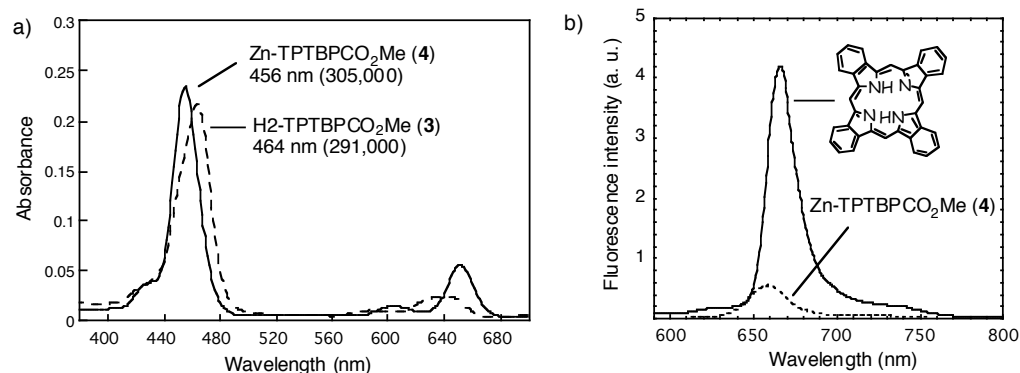
Figure 1. (a) Absorption spectra of TPTBPCO 2 Me ( 3 ) and ( 4 ) in \text{CH}_2\text{Cl}_2 . (b) Fluorescence emission of Zn-TPTBPCO 2 Me ( 4 ) compared to H2-TBP (solutions in \text{CH}_2\text{Cl}_2 with an absorbance = 0.15)
