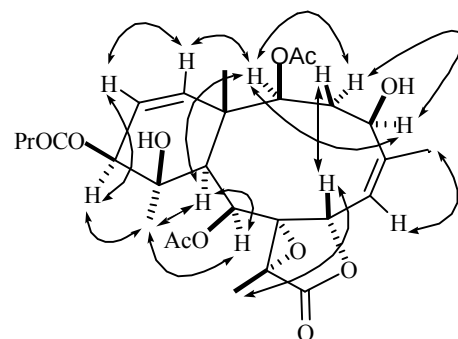
Figure 2. Selective NOESY Correlations for 1 .
