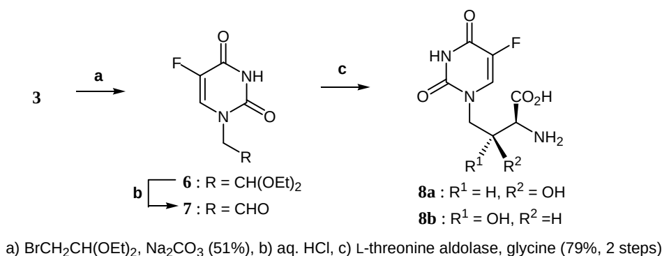
Scheme 2 Preparation of \beta -hydroxy- \alpha -L-amino acids having 5-fluorouracil residue at \gamma -position ( 8a , 8b )
