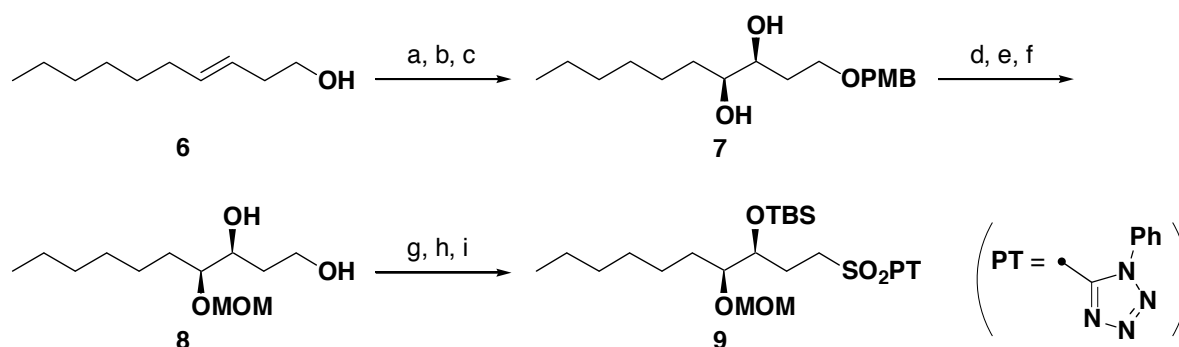
Scheme 2. a) PMBCl, NaH, TBAB, THF, reflux, quant. b) AD-mix- \alpha , t -BuOH, H 2 O, 95% e.e. c) recrystn., >99% e.e., 74% in 2 steps. d) DDQ, CH 2 Cl 2 . e) MOMCl, i -Pr 2 EtN, CH 2 Cl 2 . f) AcOH, H 2 O, THF, 81% in 3 steps. g) PTSH, PPh 3 , DIAD, THF. h) (NH 4 ) 6 Mo 7 O 24 ·4H 2 O, H 2 O 2 , EtOH. i) TBSOTf, 2,6-lutidine, CH 2 Cl 2 , 91% in 3 steps.
