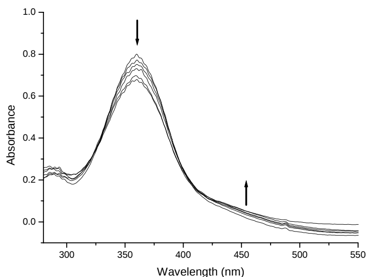
Figure 2. Absorption spectrum of 2 under irradiation conditions (365 nm: 0, 30, 60, 120, 360 and 420 s)
