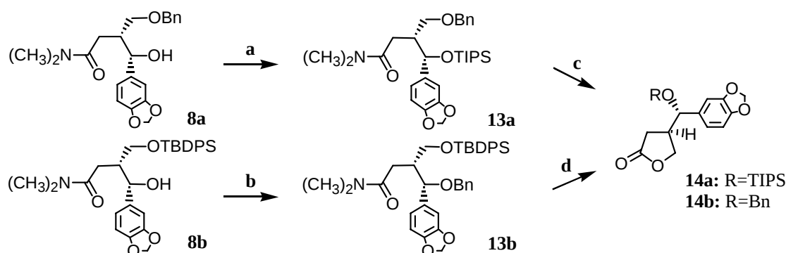
Scheme 2. Reagents and conditions: (a) TIPSOTf, 2,6-lutidine, \text{CH}_2\text{Cl}_2 , 86%; (b) BnBr, \text{Ag}_2\text{O} , \text{CH}_3\text{CO}_2\text{C}_2\text{H}_5 , 75%; (c) 1. 5% Pd/C, \text{H}_2 , \text{CH}_3\text{OH} ; 2. PPTS, toluene, 45 °C, 88% ( 14a ) (2 steps); (d) 1. (\text{C}_4\text{H}_9)_4\text{NF} , THF; 2. p -TsOH, toluene, 81% ( 14b ) (2 steps).
