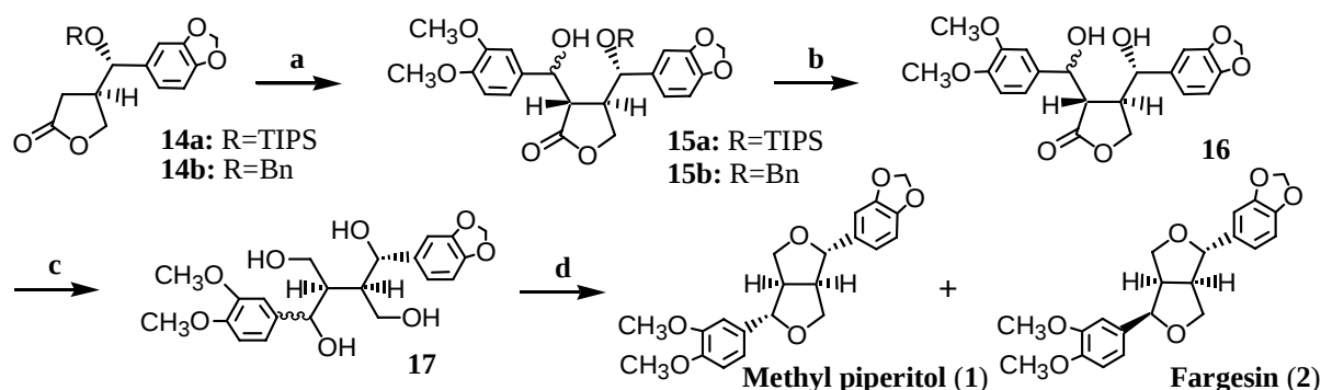
Scheme 3. Reagents and conditions: (a) \text{LiHMDS} , 3,4-dimethoxybenzaldehyde, THF, -78 °C, 77% ( 15a , 59:41), 95% ( 15b , 47:53); (b) (\text{C}_4\text{H}_9)_4\text{NF} , THF (to 15a ), 96% or 5% Pd/C, \text{H}_2 , \text{CH}_3\text{CO}_2\text{C}_2\text{H}_5 (to 15b ), 97%; (c) \text{LiAlH}_4 , THF, 87%; (d) \text{MsCl} , pyridine, \text{CH}_2\text{Cl}_2 , 38% ( 1 ), 24% ( 2 ).
