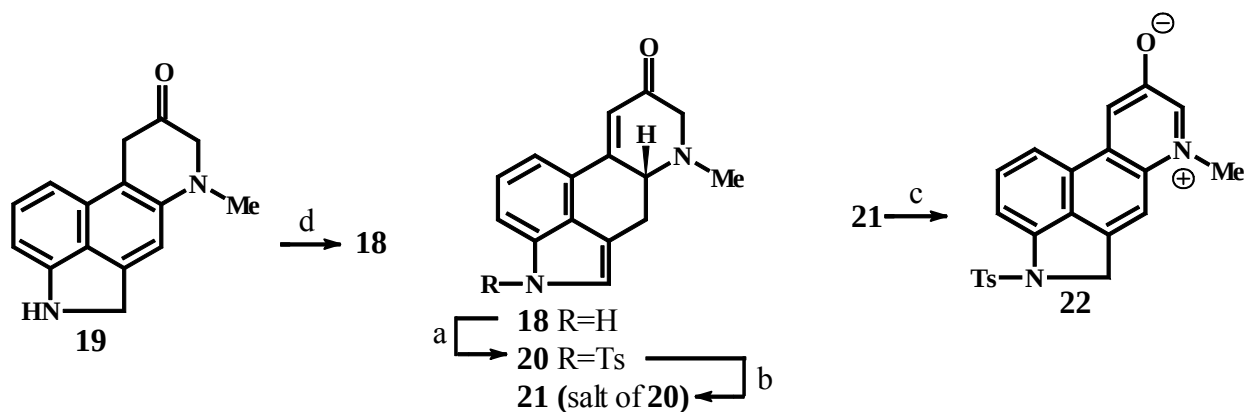
Scheme 3 -- reagents and conditions : a) \text{KOH}/\text{TsCl} , TBAHS, \text{CH}_2\text{Cl}_2 , 0^\circ\text{C} \rightarrow \text{rt} , 2 h, 66 %; b) \text{DMSO}-d_6 + \text{CF}_3\text{CO}_2\text{D} , rt, 5 min; c) after 4-5 weeks; d) ref. 19.
