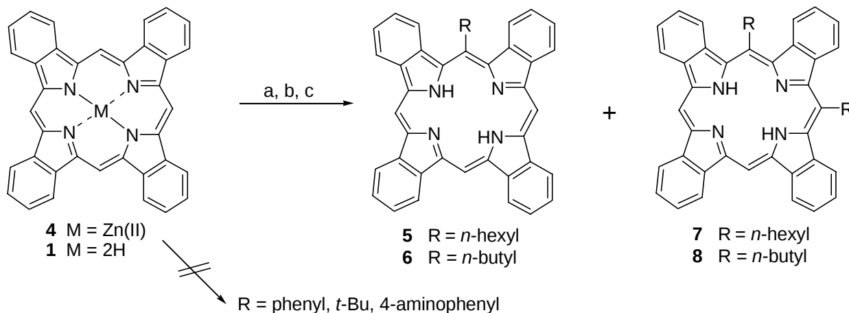
Scheme 1. Reactions of (tetrabenzoporphyrinato)zinc(II). a) \text{LiR}^1 , THF, -30 to -80 °C; b) \text{H}_2\text{O} , 10 min; c) DDQ, 1 h.
