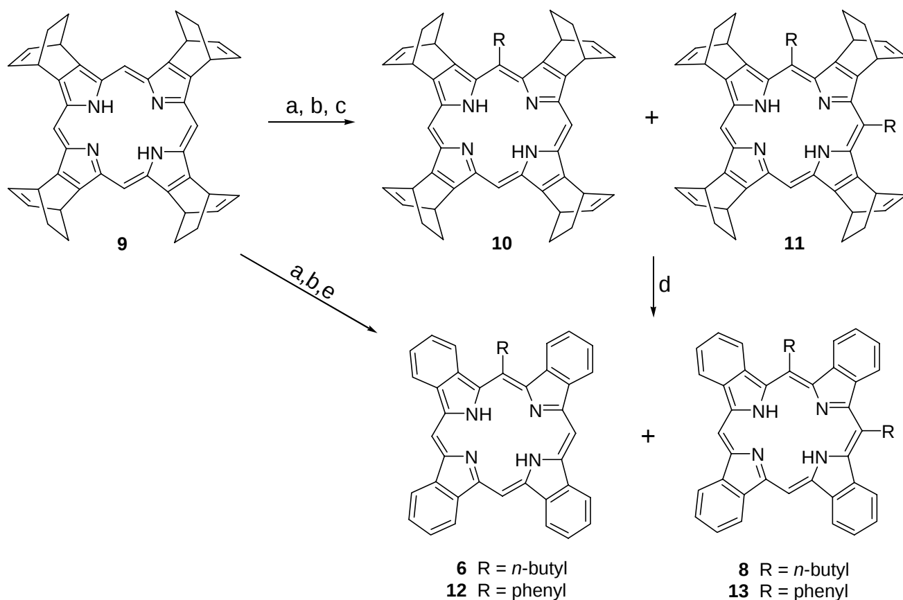
Scheme 2. Reactions of the benzoporphyrin precursor 9 . a) \text{LiR}^1 , THF, -30 to -80 °C; b) \text{H}_2\text{O} , 10 min; c) air, 18 h; d) DDQ, 1 h; e) DDQ, 200 °C, 1 h.
