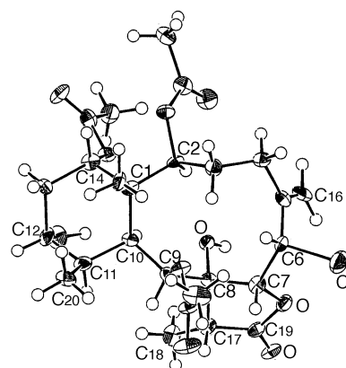
Figure 2. ORTEP representation of 3 .
