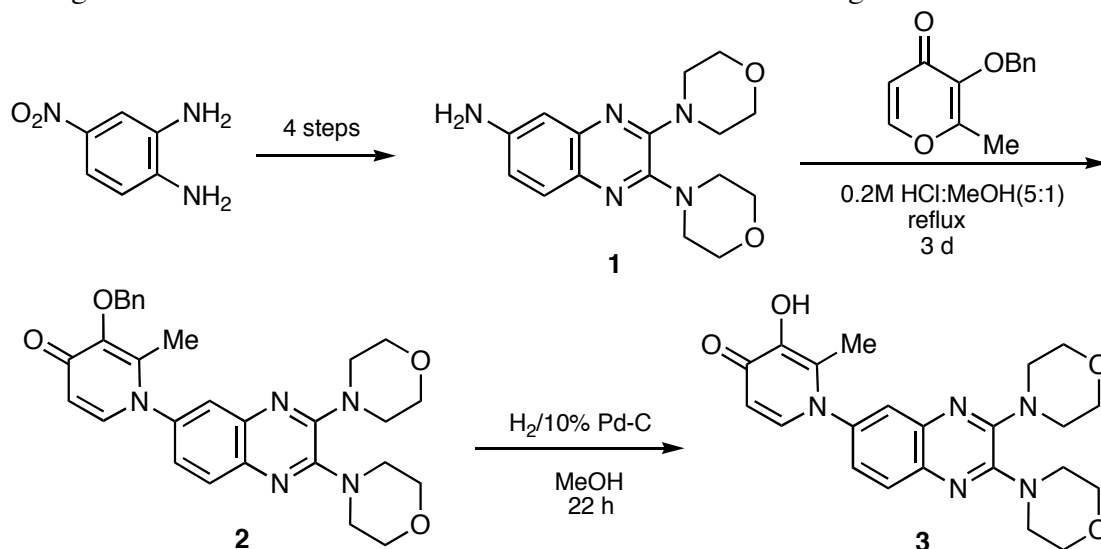
Scheme 2 Synthesis of 3-hydroxy-2-methyl-1-(2,3-dimorpholinoquinoxalin-6-yl)pyridin-4(1 H )-one
