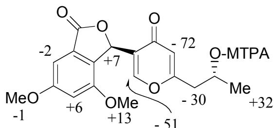
Figure 1. Differences of chemical shifts ( \Delta\delta in Hz) between the ( S )- and ( R )-MTPA esters of 3
