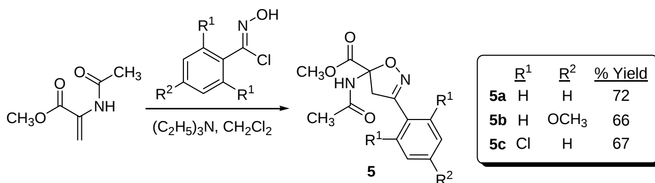
Scheme 5
