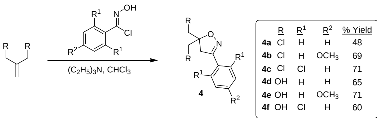
Scheme 4
