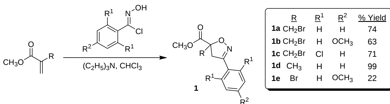
Scheme 2
