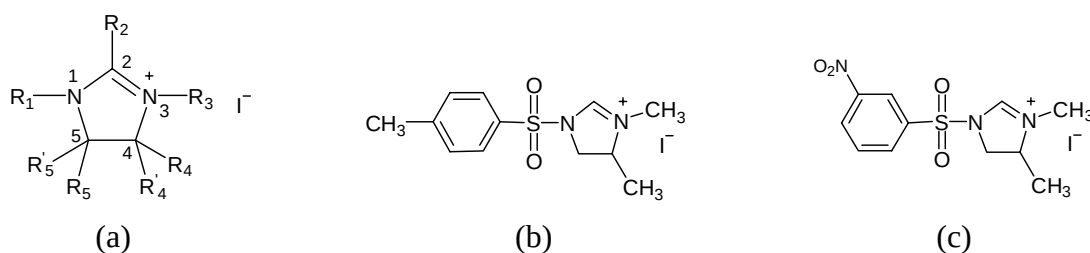
Figure 1 (a) General tetrahydrofolate coenzyme models. (b) 1-Tosyl-3,4-dimethylimidazolinium iodide ( 1 ). (c) 1-(3-nitro-benzenesulfonyl)-3,4-dimethylimidazolinium iodide ( 2 )
