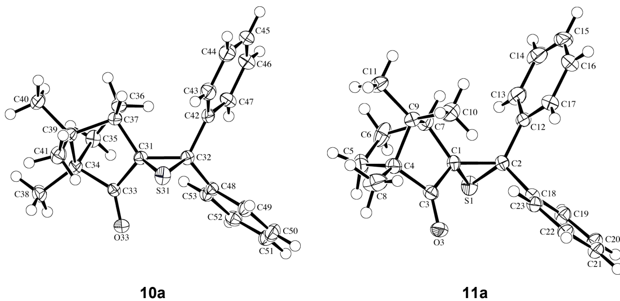
Figure 1. ORTEP plot 13 of the molecular structure of the two stereoisomeric thiranes ( 10a ) and ( 11a ) (50% probability ellipsoids; arbitrary numbering of atoms).
