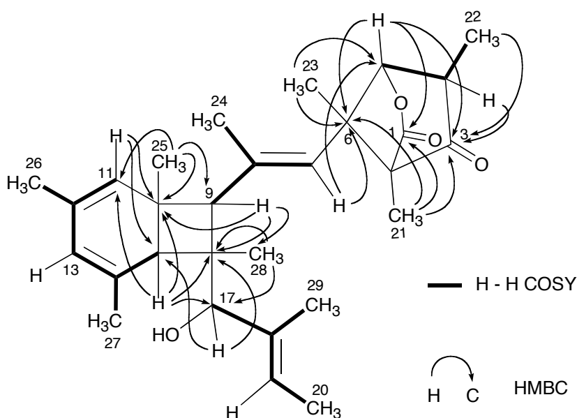
Figure 1. COSY and key HMBC correlations for shimalactone B ( 2 )
