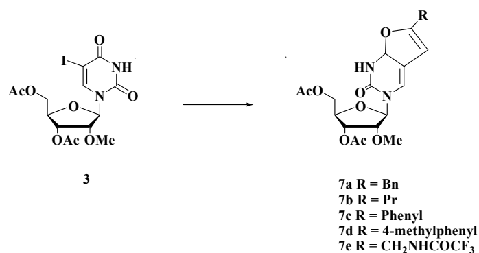
Scheme 2 Synthesis of 2- O' -methyl cyclic furofused pyrimidine nucleoside derivatives
