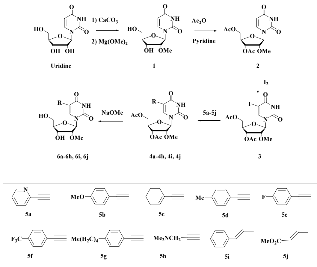
Scheme 1 Synthesis of 2'- O -methyl-5-alkynyl and 5-alkenyl substituted uridines
