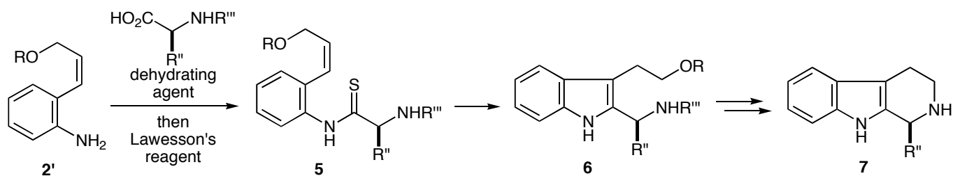
Scheme 2. Synthesis of Tetrahydro- \beta -carboline from 2-Alkenylthioanilides derived from \alpha -Amino Acids.
