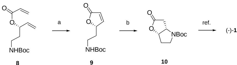
Scheme 2. Reagents and conditions: (a) Grubbs' 2nd generation Ru catalyst, CH 2 Cl 2 , 40°C (85%); (b) NaH, DMF, 0°C (96%).
