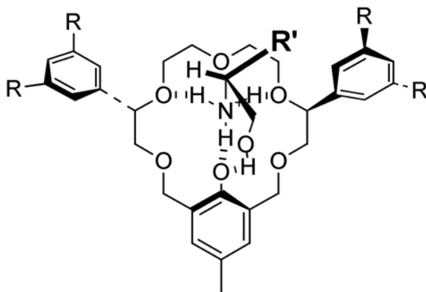
Figure 4. Predicted geometries of complexes of ( S,S )- 1 ( R=CH_3 ) and ( S,S )- 3 ( R=H ) with ( R )- 5–7 ( R'=CH_3 , Ph, i -Pr).
