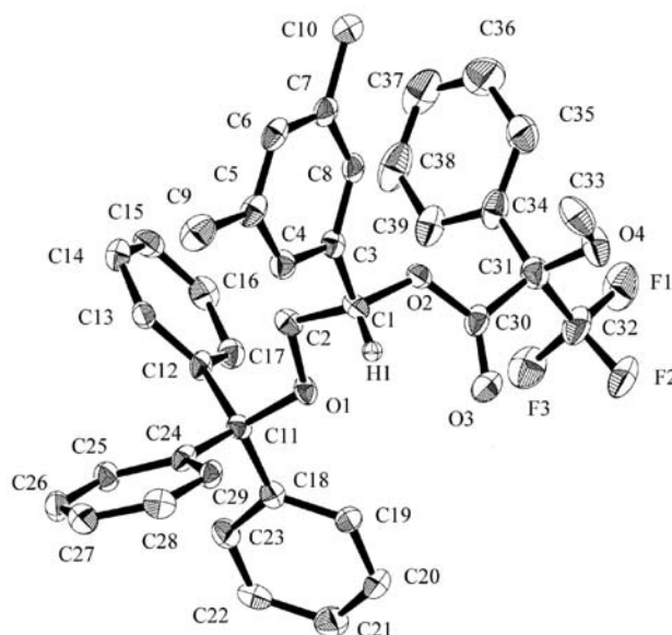
Figure 3. An ORTEP view of the ( R )-MTPA ester of (+)- 10 . All hydrogen atoms except the one attached to the stereocenter are omitted for clarity.
