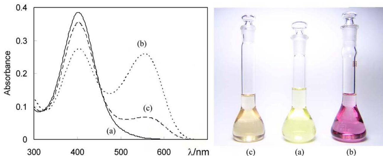
Figure 5. UV-VIS spectra and corresponding pictures: (a) A chloroform solution of ( S,S )- 1 ( 1.85 \times 10^{-5} M) at 25 °C (solid line); (b) The same solution as (a) containing 2 equivalent of ( R )- 6 (dotted line); (c) The same solution as (a) containing 2 equivalent of ( S )- 6 (dashed line).
