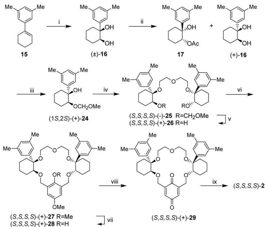
Scheme 2. Synthesis of (S,S,S,S)- 2 : Reagents i. 1) HCO 3 H, 2) aq. NaOH ii. Lipase QL, CH 2 =C(Me)OAc, Cyclohexane iii. CH 2 (OMe) 2 iv. TsOCH 2 CH 2 OCH 2 CH 2 OTs, NaH, THF v. HCl, MeOH vi. 1,3-bisbromomethyl-2,5-dimethoxybenzene, NaH, THF vii. EtSNa, DMF viii. Ce(NH 4 ) 2 (NO 3 ) 6 , MeCN ix. 2,4-dinitrophenylhydrazine, H 2 SO 4 , EtOH
