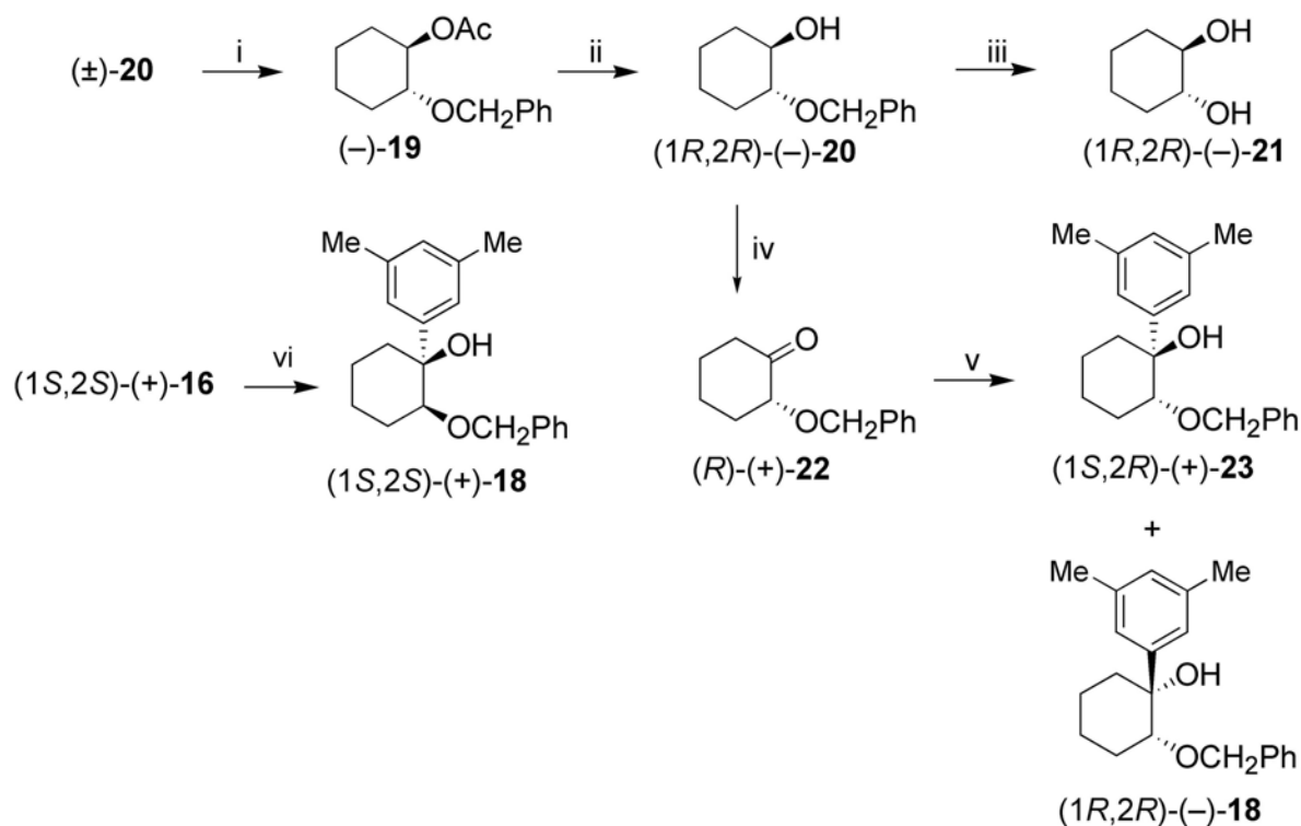
Scheme 3. Synthetic pathway of (+/–)- 18 : Reagents i. Lipase YS, CH 2 =C(Me)OAc, iso -Pr 2 O ii. KOH, MeOH, H 2 O iii. H 2 , 10% Pd/C iv. Jones' reagent v. 3,5-dimethylphenyl magnesium bromide vi. C 6 H 5 CH 2 Br, NaH, THF.
