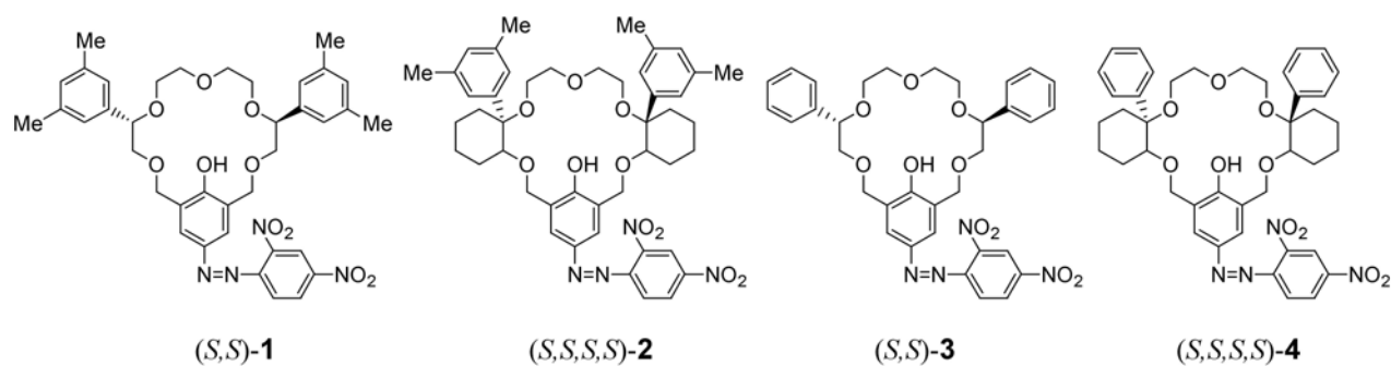
Figure 1. List of host molecules
