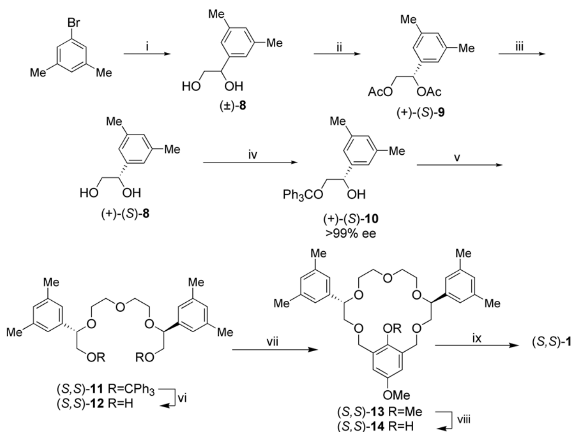
Scheme 1. Synthesis of (S,S)- 1 : Reagents i. 1) Mg, Et 2 O, 2) CH 2 =CHBr, NiCl 2 (dppp), 3) OsO 4 , N -methylmorpholine- N -oxide, H 2 O ii. Lipase QL, CH 2 =C(Me)OAc, Cyclohexane iii. K 2 CO 3 , MeOH, H 2 O iv. 1) Ph 3 CCl, DMAP, Et 3 N, DMF 2) Recrystallization from CHCl 3 -EtOH v. TsOCH 2 CH 2 OCH 2 CH 2 OTs, NaH, THF vi. HCl, MeOH vii. 1,3-bis(bromomethyl)-2,5-dimethoxybenzene, NaH, THF viii. EtSNa, DMF ix. 1) Ce(NH 4 ) 2 (NO 3 ) 6 , MeCN 2) 2,4-dinitrophenylhydrazine, H 2 SO 4 , EtOH.
