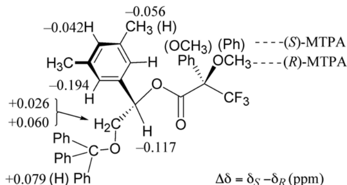
Figure 2. Chemical shift differences (ppm) between the diastereomeric ( R )- and ( S )-MTPA esters of (+)- 10 obtained from their 1 H-NMR (270MHz, 30°C, CDCl 3 ).
