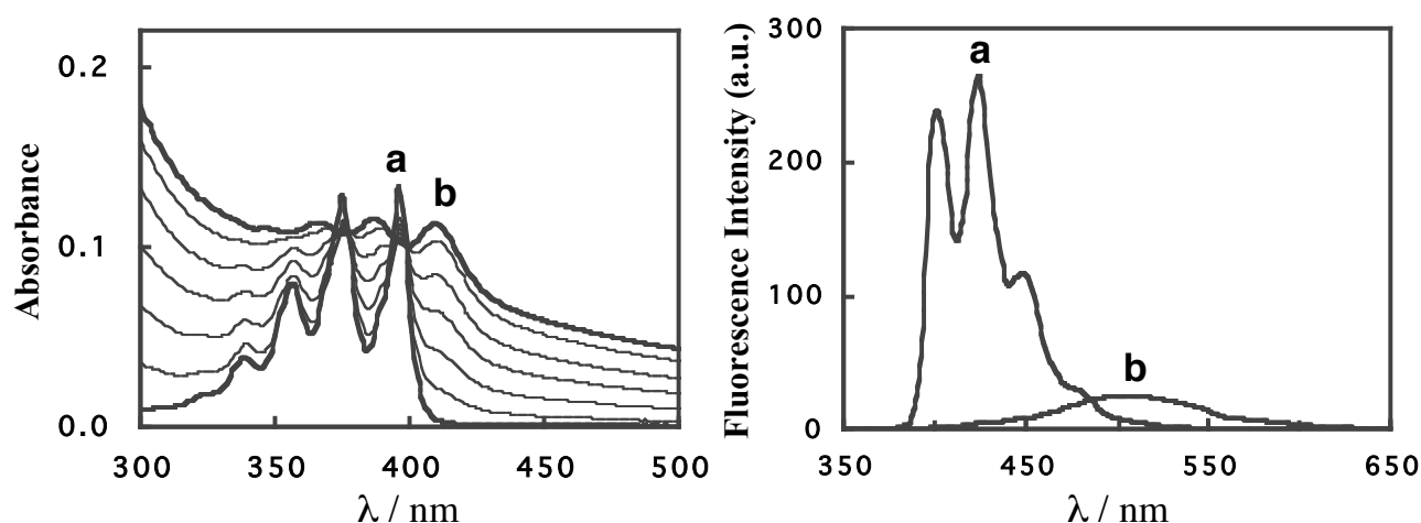
Figure 3. Absorption (10 \mu\text{M} ) and fluorescence (10 \mu\text{M} , excited at 335 nm) spectra of 3 in MeCN without n\text{-Bu}_4\text{N}^+\text{H}_2\text{PO}_4^- (a) and with 2.5 equiv. of n\text{-Bu}_4\text{N}^+\text{H}_2\text{PO}_4^- (b), respectively.
