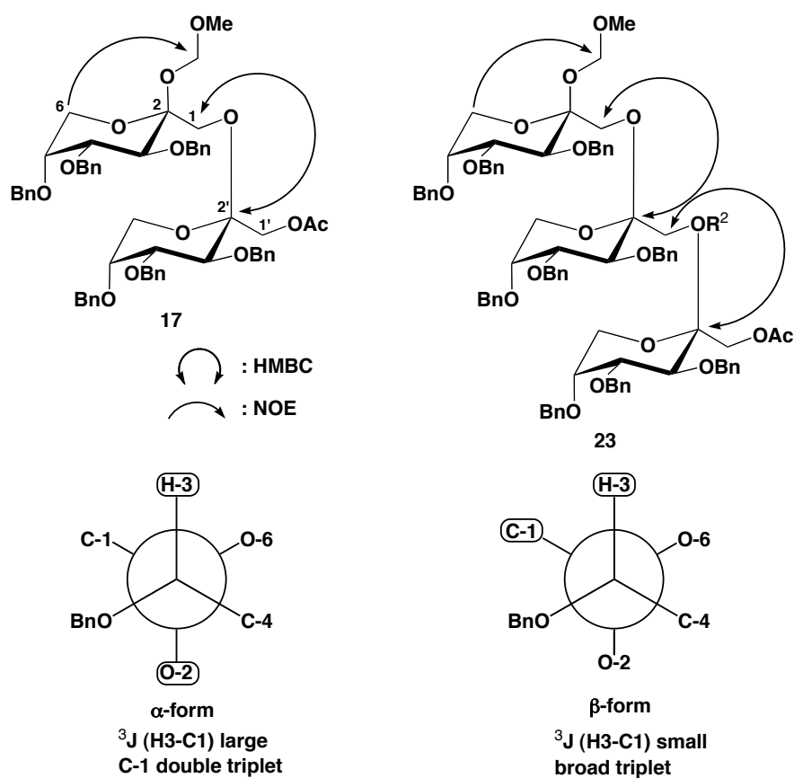
Figure 1. Structure Elucidation of Fructosyl oligosaccharides
