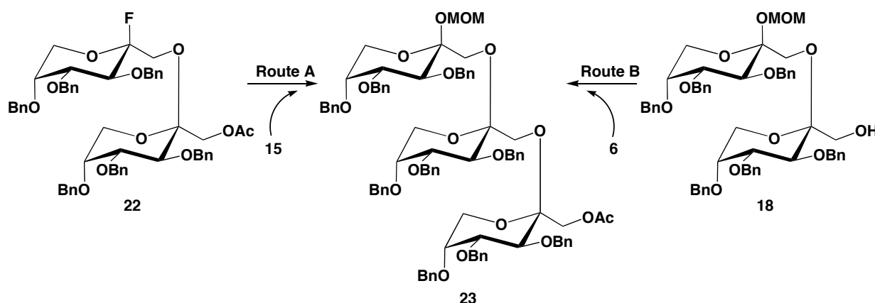
Scheme 3. Synthesis of Fructopyranosyl-β(2→1)-trisaccharide ( 23 )
