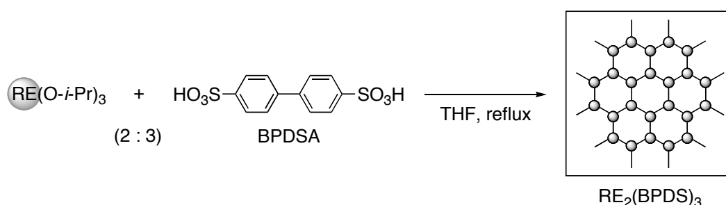
Scheme 2. Preparation of the coordinated polymer catalysts
