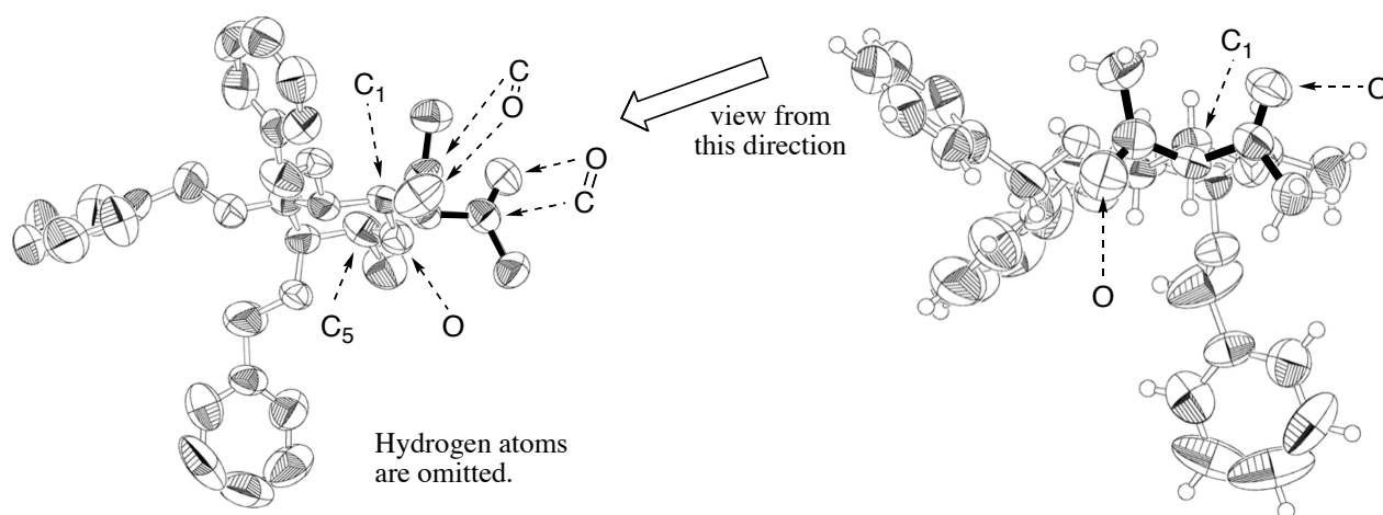
Figure 2. ORETP drawing of 10 \beta -keto ( \beta -diketone framework is drawn by bold lines).
