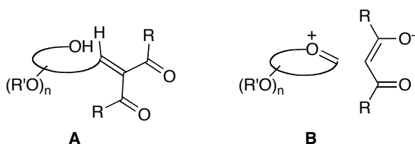
Figure 1. Isomerization of the anomeric stereochemistry.
