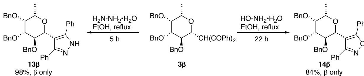
Scheme 2. Reaction of C -fucosylated diketone ( 3 \beta ) with hydrazine or hydroxylamine.
