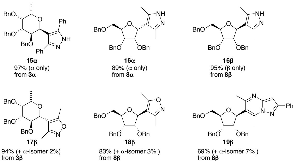
Figure 3. Selected examples of heterocyclic construction from C -glycosyl \beta -diketones.
