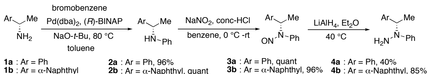
Scheme 1 Synthesis of hydrazines ( 4 )
