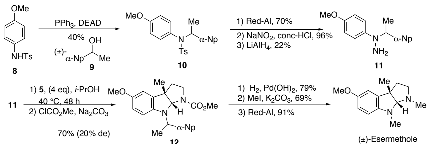
Scheme 3 Synthesis and reaction of 11 , and conversion to (±)-esermethole
