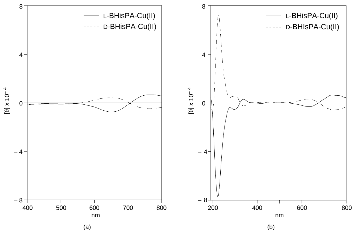
Figure 2. (a) CD spectra of L-BHisPA-Cu(II) and D-BHisPA-Cu(II) in a solid state as nujol mulls and (b) in methanol solution ( 1.0 \times 10^{-4} M).
