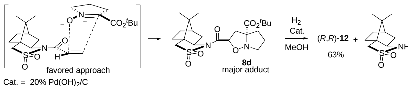
Scheme 4.
