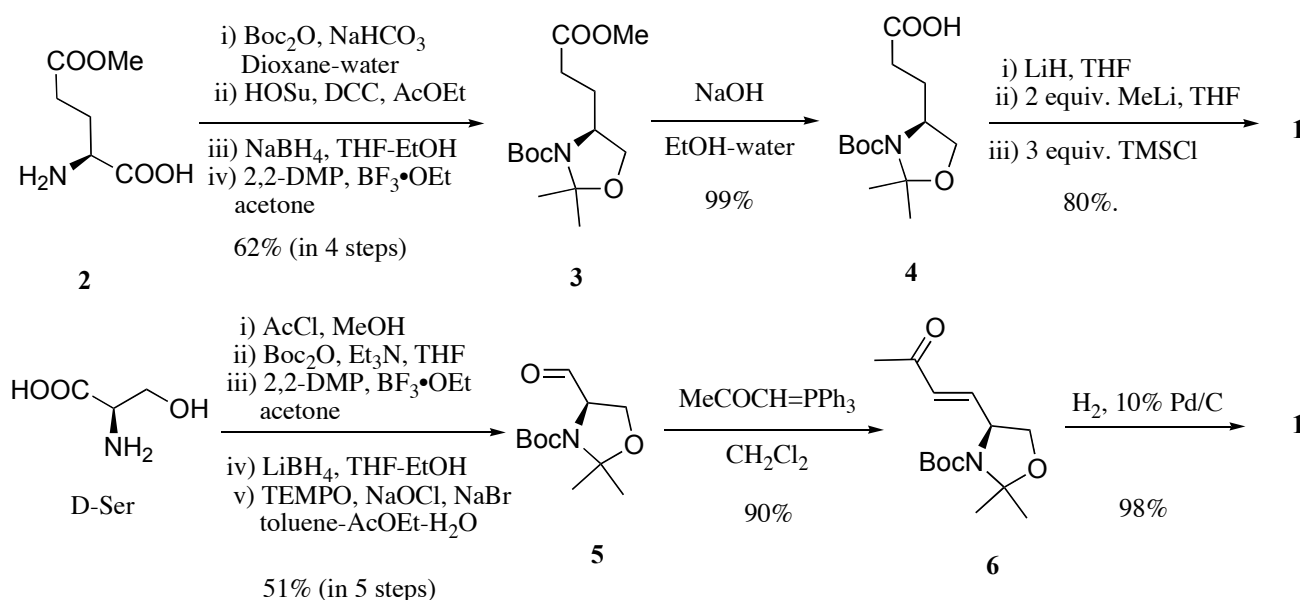
Scheme 2. Synthesis of methyl ketone ( 1 ) from \gamma -methyl glutamate or D-serine
