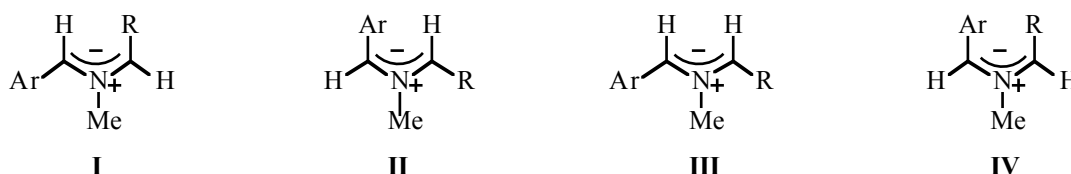
Figure 2 Four possible azomethine ylide configurations
