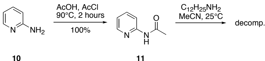
Scheme 6. Reactivity of 2-acetamidopyridine
