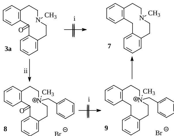
Scheme 2. Reagents and conditions: (i) LiAlH 4 -AlCl 3 , NaBH 4 -AlCl 3 , LiAlH 4 -pyridine, or H 2 -PtO 2 , respectively; (ii) benzyl bromide, 24 h, 70 °C, 60 %.
