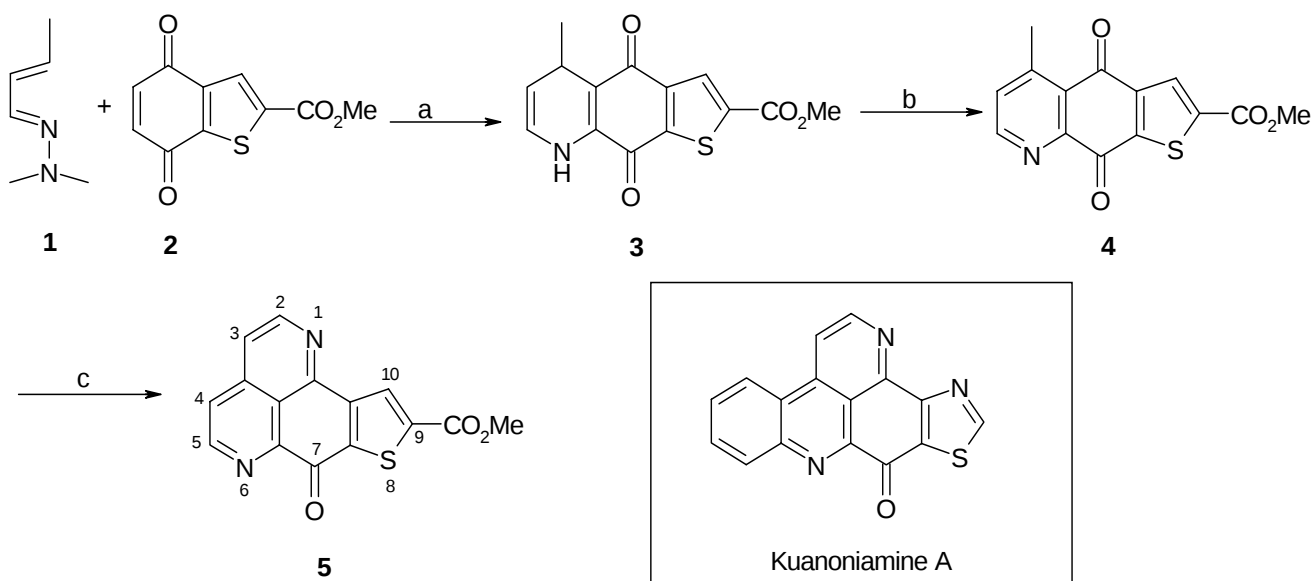
Scheme 1 Reagents: a) \text{CH}_3\text{CN} , \text{Ac}_2\text{O} b) \text{PCC-Al}_2\text{O}_3 , \text{CH}_2\text{Cl}_2 c) \text{DMF-DEA} , \text{DMF} , \text{NH}_4\text{Cl} , \text{AcOH} .
