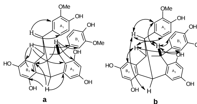
Figure 2. Key HMBC (a) and NOE (b) Interactions of 2
