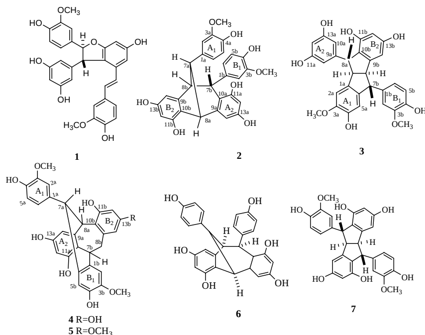
Figure 1. Structures of Compounds ( 1-7 )
