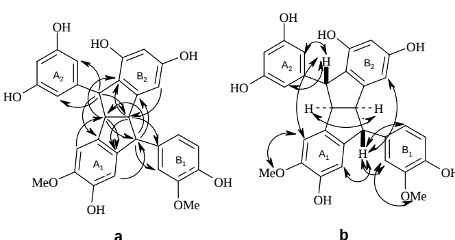
Figure 3. Key HMBC (a) and NOE (b) Correlations of 3
