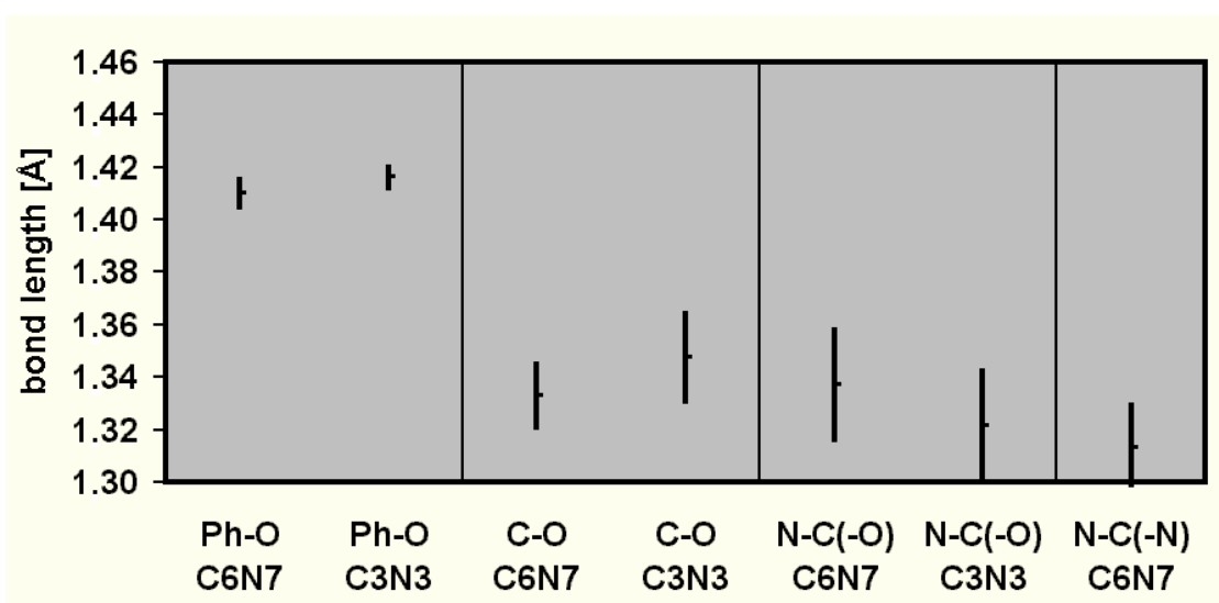
Figure 4: Comparison of maximum, minimum, and average bond lengths as observed in C_6N_7(OPh)_3 and C_3N_3(OPh)_3 . Error (not shown) \approx \pm 0.03 Å
