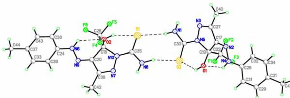
Figure 2. Two crystallographically independent molecules in X-Ray structure of 5-(pyrazolinyldiazeno)azole ( 4g )
