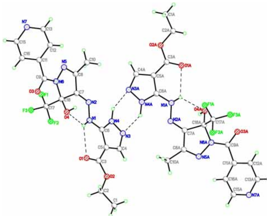
Figure 1. Two crystallographically independent molecules in X-Ray structure of 5-(pyrazolinyldiazeno)azole ( 4e )
