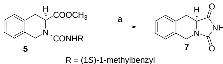
Scheme 2. (a) \text{CF}_3\text{COOH} , 84%.
