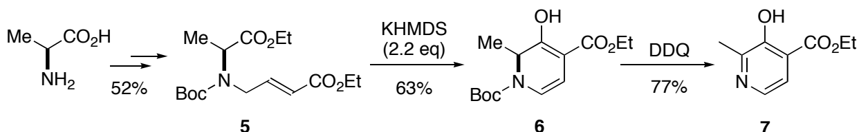
Scheme 5
