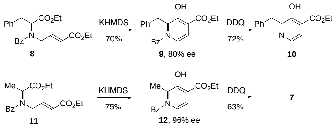
Scheme 6
