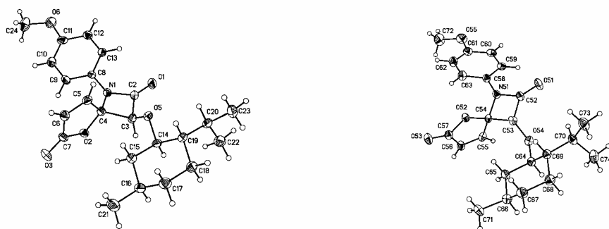
Figure 2b X-Ray structure of compounds (3S,4S,1'R,2'S,5'R)\text{-8c} and (3R,4R,1'R,2'S,5'R)\text{-8c}
