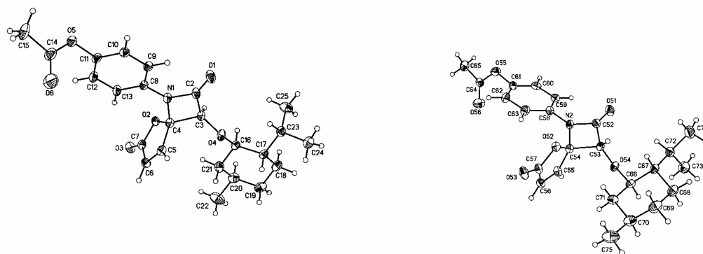
Figure 2a X-Ray structure of compounds (3S,4S,1'R,2'S,5'R)\text{-8b} and (3R,4R,1'R,2'S,5'R)\text{-8b}
