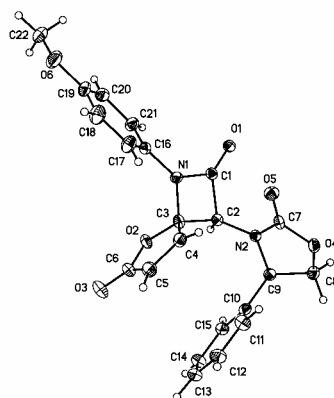
Figure 4 X-Ray structure of compound (3 S ,4 S ,4' R )-(11b)
