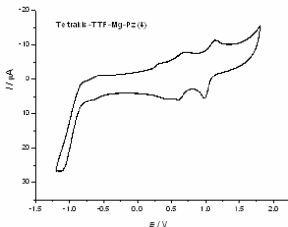
Figure 4. Cyclic voltammogram of 4 , in 0.1M tetrabutylammonium hexafluorophosphate in \text{CH}_2\text{Cl}_2/\text{CH}_3\text{CN}(5/1, \text{v/v}) at 0.1 \text{ V s}^{-1} , Pt electrode.
